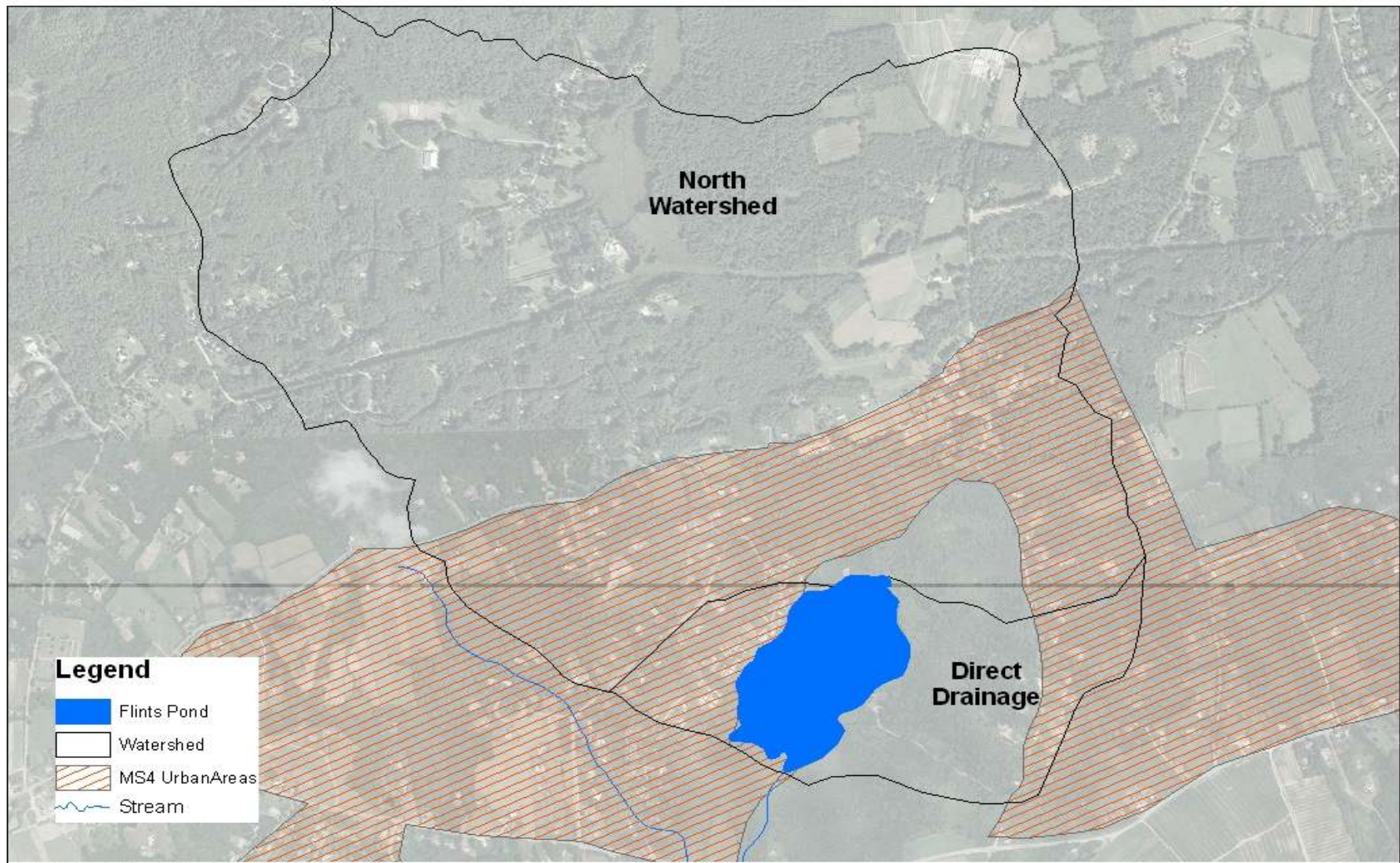
FIGURE 5-1 MS4 Urbanized Areas Flint's Pond Hollis, NH
